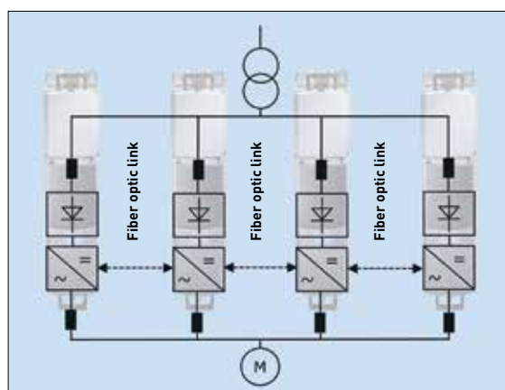
Example of the DriveSynch configuration.
