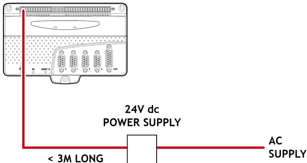
Motion Coordinator with dedicated power source
